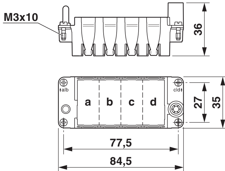
Dimensional drawing
