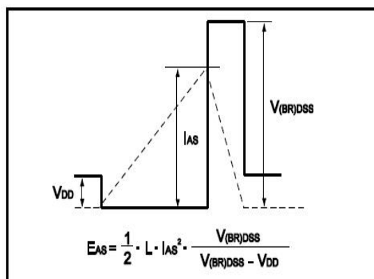
Fig.12 Avalanche Waveform
