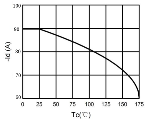
Figure 4. Drain Current
