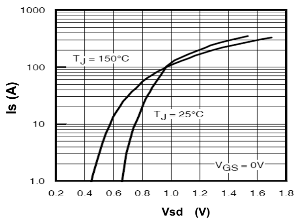
Figure 9. Body-Diode Characteristics
