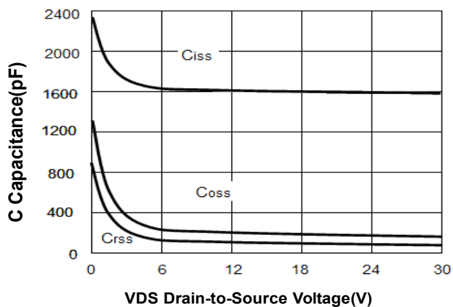
Figure 8. Capacitance
