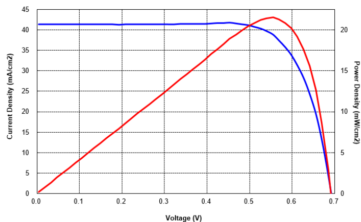
Current-Voltage Characteristics
