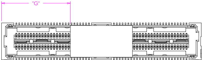
LOCATION OF PPP-51 FOR POSITIONS -052 & -104 [CENTERED IN PART]
