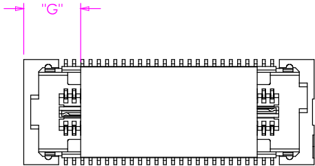
LOCATION OF PPP-51 FOR POSITIONS -026, -078 & -130 [CENTERED IN MIDDLE OF BANK CLOSEST TO MIDDLE OF PART]
