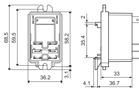
066.07 with relay
