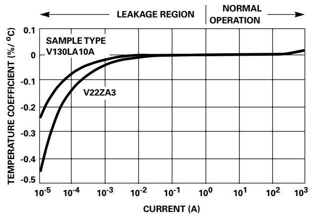
NOTE: Typical Temperature Coefficient of Voltage vs Current, 14mm Size, 55°C to 125°C.
