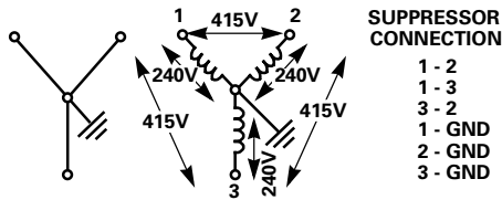
FIGURE 25F. 3 PHASE 240V/415V
