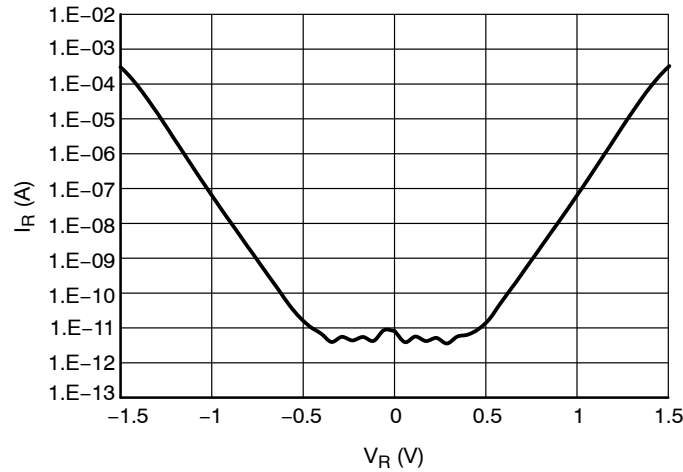
Figure 3. IV Characteristics
