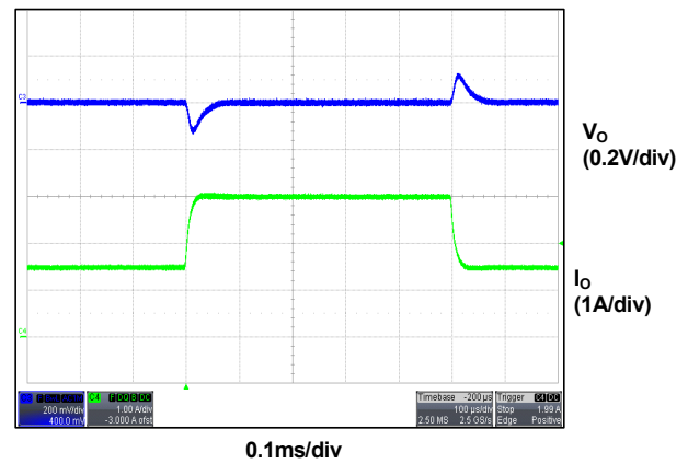
Figure 9. 50% to 100% Load Transient
