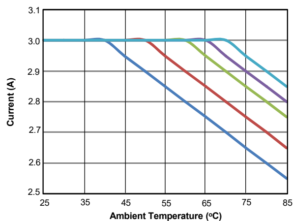
Figure 11. Thermal Derating Curve with 12VIN
