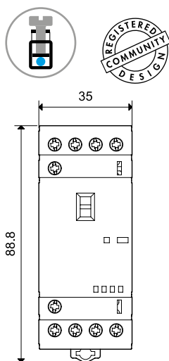
Type 22.34 Box clamp
