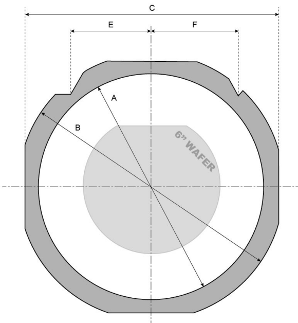
Figure 11 FF108 Frame with a 6 inch wafer
