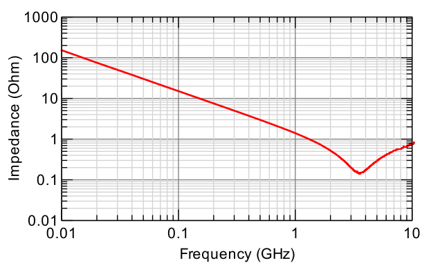
Figure 2 - 100pF WLSC measurement results (Impedance characteristic versus Frequency in shunt mode)
