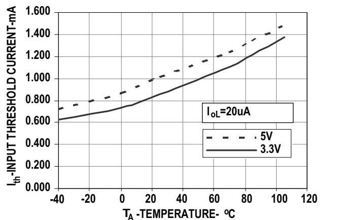
Figure 2: Typical Input Threshold Current vs. Temperature
