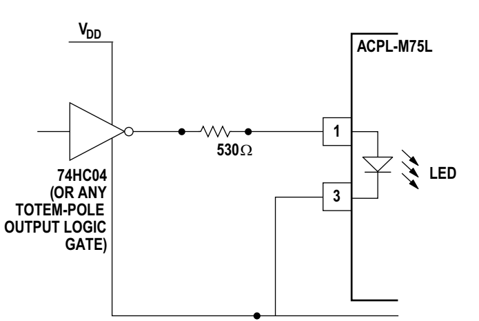
Figure 17: CMOS Gate Drive Circuit for ACPL-M75L Families
