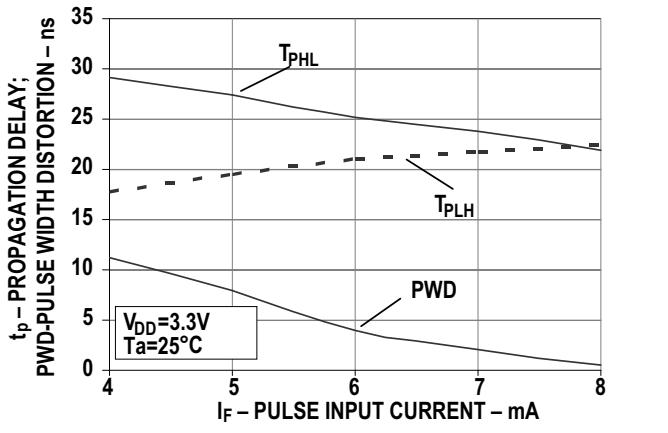
Figure 6: Typical Switching Speed vs. Pulse Input Current at 3.3V Supply Voltage
