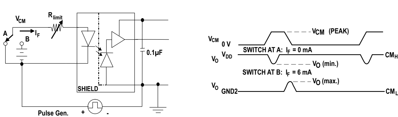
Figure 18: Test Circuit for Common Mode Transient Immunity and Typical Waveforms
