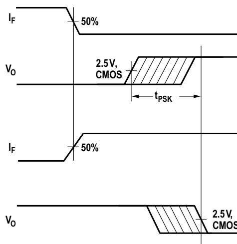
Figure 10: Parallel Data Transmission Example
