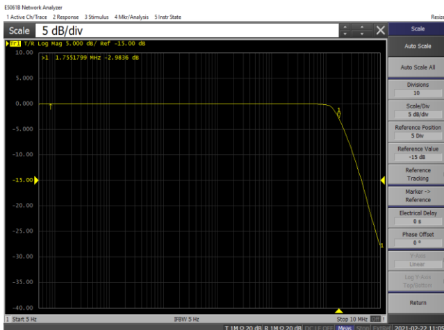
Figure 7. -3dB Bandwidth, G = 1 , V_s = 30V
