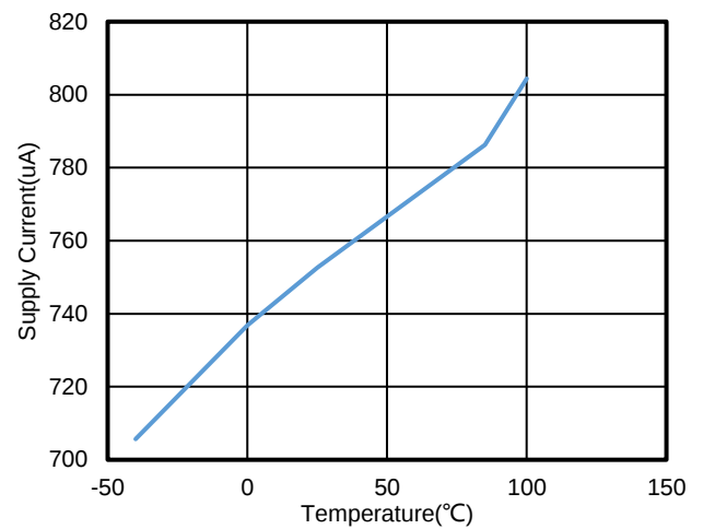
Figure 4. I_q vs. Temperature, \pm 15V Supply, TPA2642
