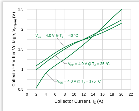
Figure 3. Collector-Emitter Voltage vs. Collector Current
