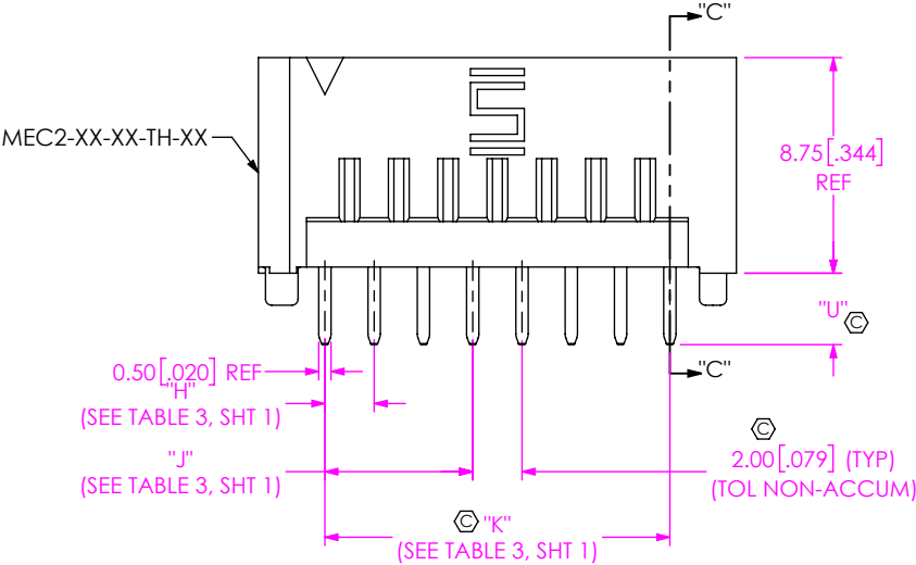
FIG 7 SCALE 3:1 MEC2-08-01-L-TH1-XX SHOWN (SAME AS FIG 1, EXCEPT AS SHOWN)
