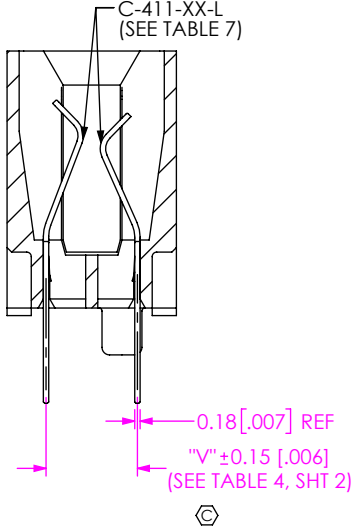
FIG 5 SCALE 1:1 (MEC2-50-01-XX-DV-XX SHOWN) (SAME AS FIG 1, EXCEPT AS SHOWN) (SOME CENTER FEATURES REMOVED FOR CLARITY)
