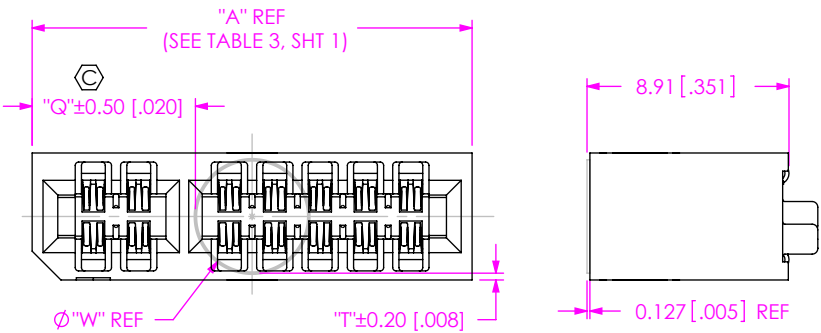
FIG 3 -K OPTION (MEC2-08-01-XX-DV-K SHOWN)
