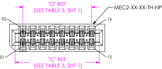
FIG 4 (MEC2-08-01-XX-XXX-NP SHOWN) (SAME AS FIG. 1, EXCEPT AS SHOWN)
