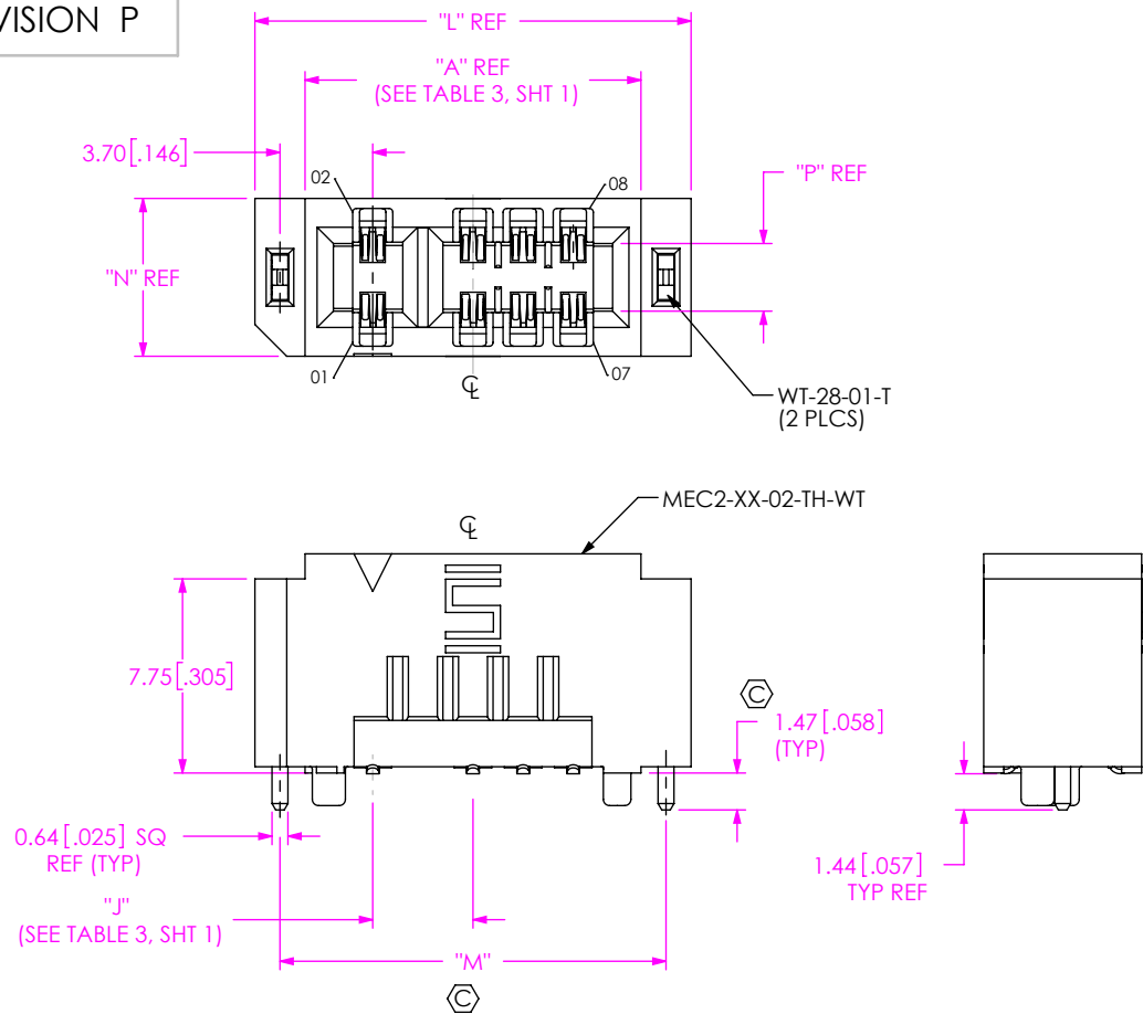
FIG 2 (MEC2-05-02-XX-DV-WT SHOWN) (SAME AS FIG. 1, EXCEPT AS SHOWN)
