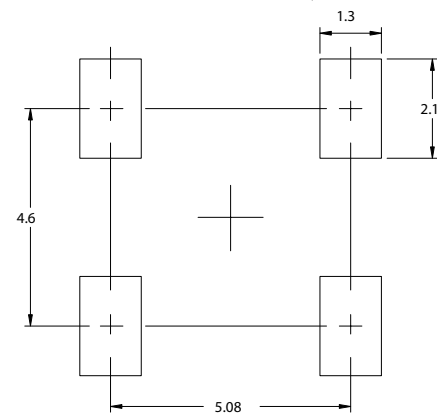
RECOMMENDED SOLDERING PATTERN
