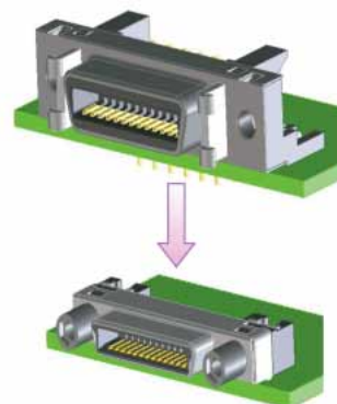
Mating Face Area Approximately 50% Reduced
