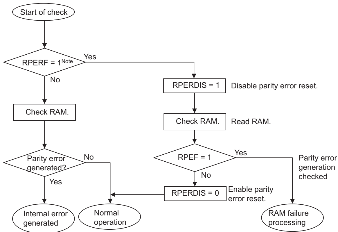
Figure 23-8. Flowchart of RAM Parity Check
