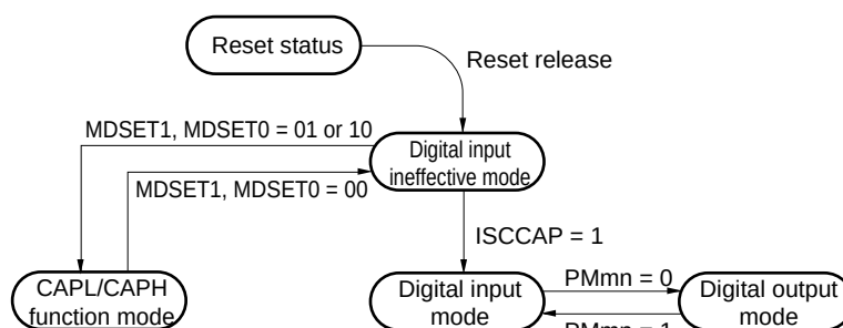
Figure 14-10. CAPL/P126 and CAPH/P127 Pin Function Status Transitions
