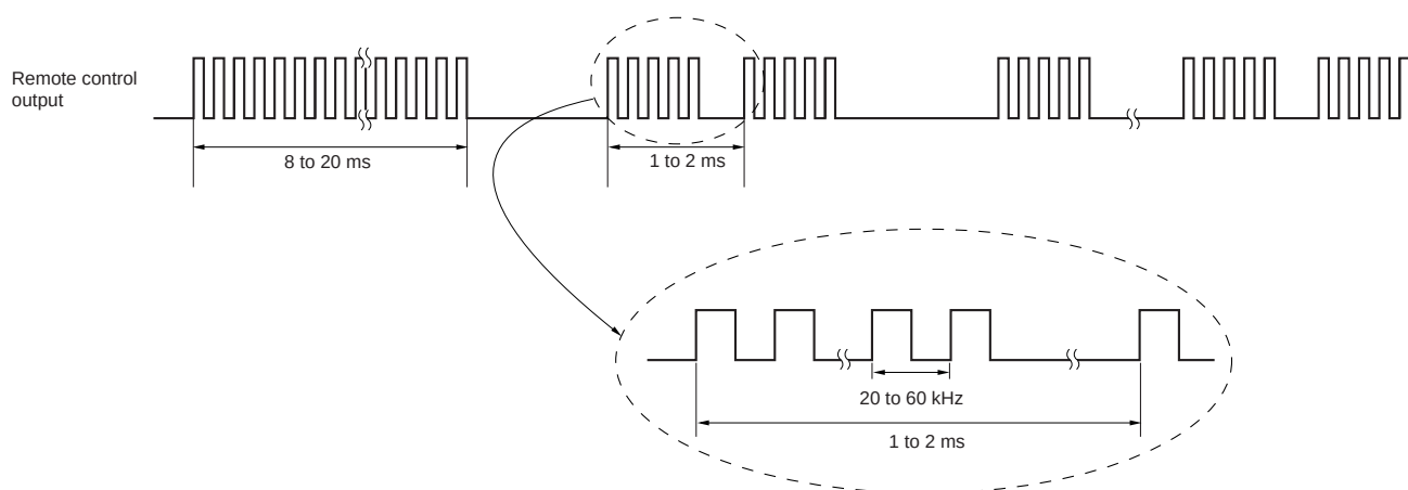
Figure 6-84. Remote Control Output
