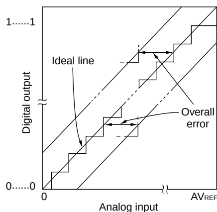
Figure 11-33. Overall Error
