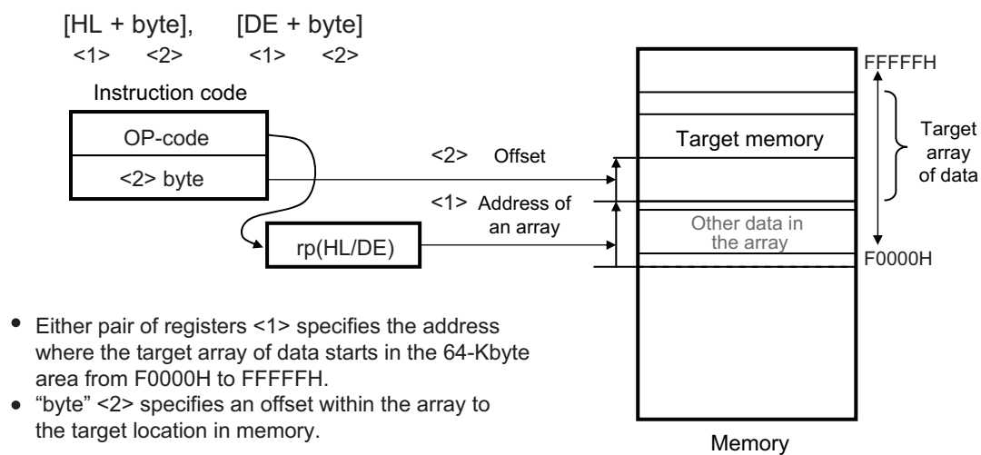
Figure 3-26. Example of [HL + byte], [DE + byte]
