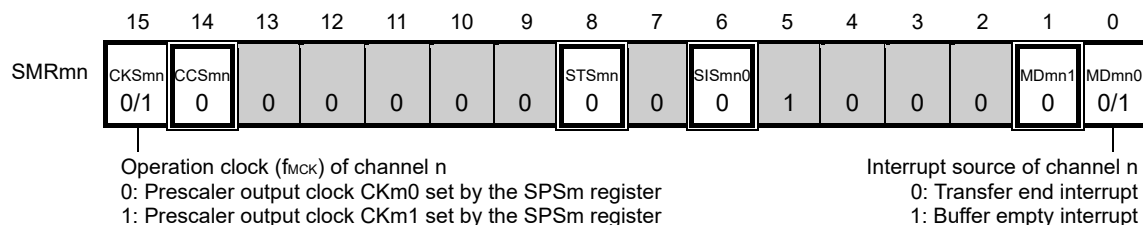
Figure 12-31. Example of Contents of Registers for Master Reception of simplified SPI (CSI00, CSI01) (1/2)
