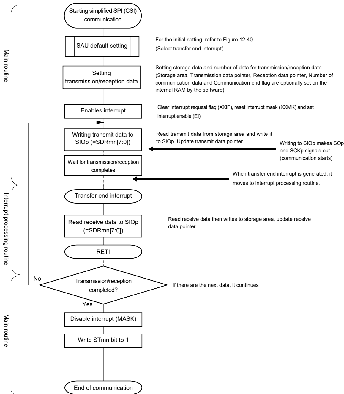
Figure 12-44. Flowchart of Master Transmission/Reception (in Single- Transmission/Reception Mode)
