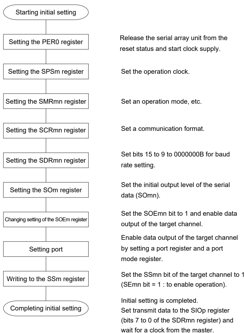
Figure 12-62. Initial Setting Procedure for Slave Transmission/Reception
