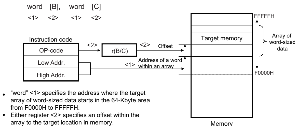
Figure 3-27. Example of word[B], word[C]
