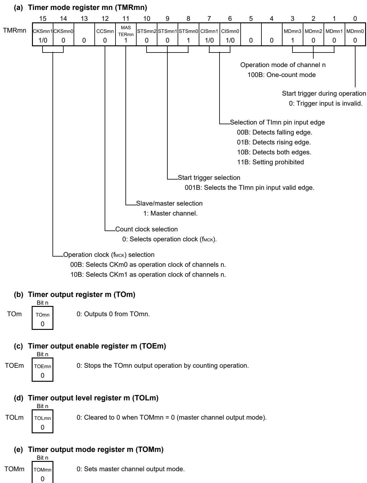
Figure 6-71. Example of Set Contents of Registers When One-Shot Pulse Output Function Is Used (Master Channel)
