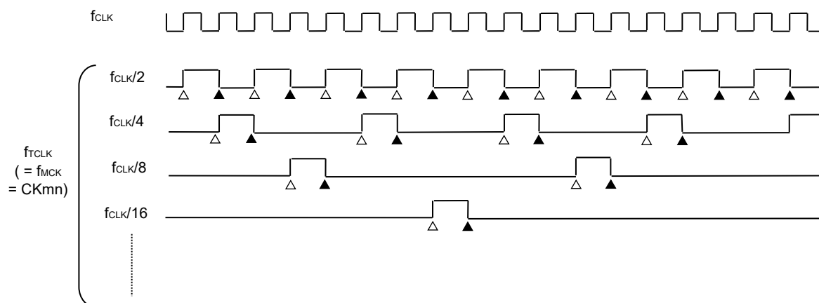
Figure 6-26. Timing of f_{\text{CLK}} and count clock ( f_{\text{CLK}} ) (When CCSmn = 0)
