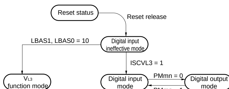
Figure 14-9. V_{L3} /P125 Pin Function Status Transitions
