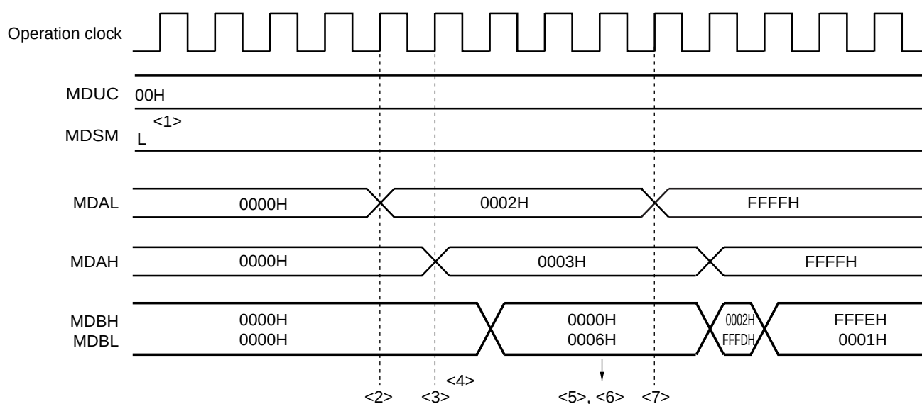
Figure 15-6. Timing Diagram of Multiplication (Unsigned) Operation ( 2 \times 3 = 6 )
