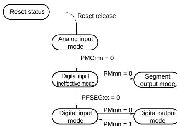
Figure 14-13. ANLxx/SEGxx/Port Pin Function Status Transitions
