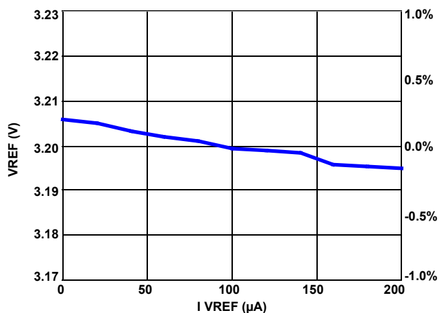
FIGURE 6. VREF LOAD REGULATION
