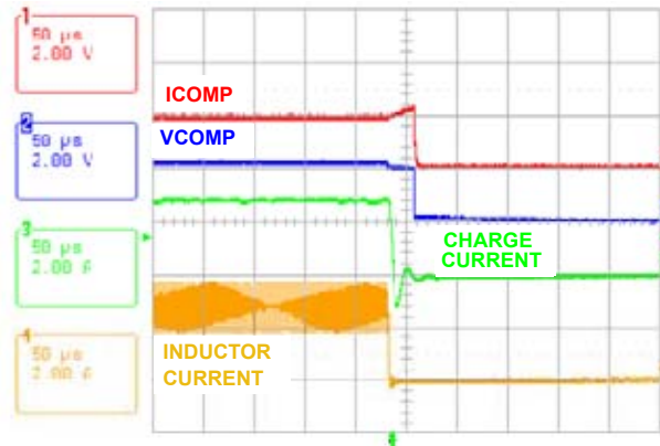
FIGURE 10. CHARGE DISABLE
