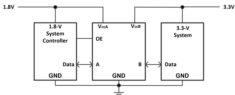
Fig.10-1. Typical Application Schematic
