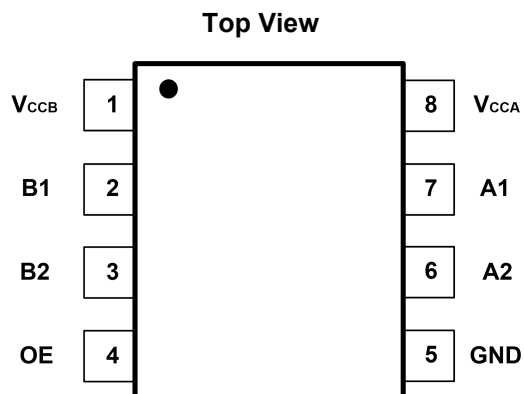
Fig.4-1. SL0102: S8 (SOT23-8) Package
