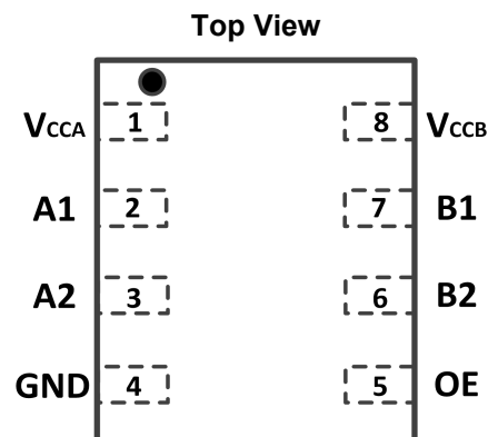
Fig.4-2. SL0102: D8 (DFN-1.4x1-8L) Package
