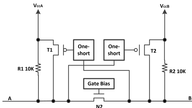
Fig.9-1. Architecture of SL0102
