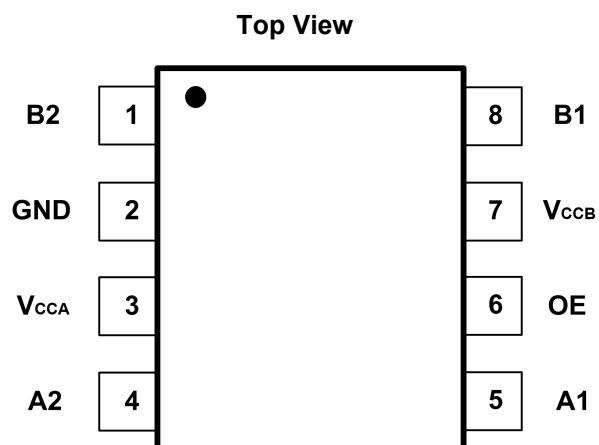
Fig.4-3. SL0102: V8 (VSSOP8) Package
