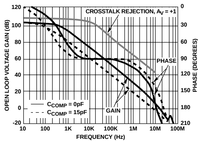
FIGURE 6. OPEN LOOP FREQUENCY AND PHASE RESPONSE
