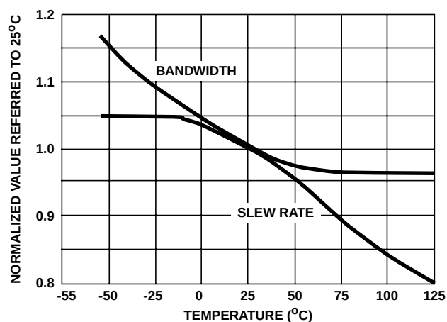
FIGURE 4. NORMALIZED AC PARAMETERS vs TEMPERATURE
