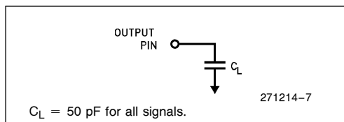
Figure 9. AC Test Load
