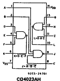
Fig. 1 - Functional diagrams.
