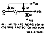
Fig. 1 - Functional diagrams.
