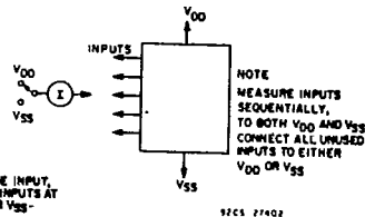
Fig. 21 — Input leakage current test circuit.
