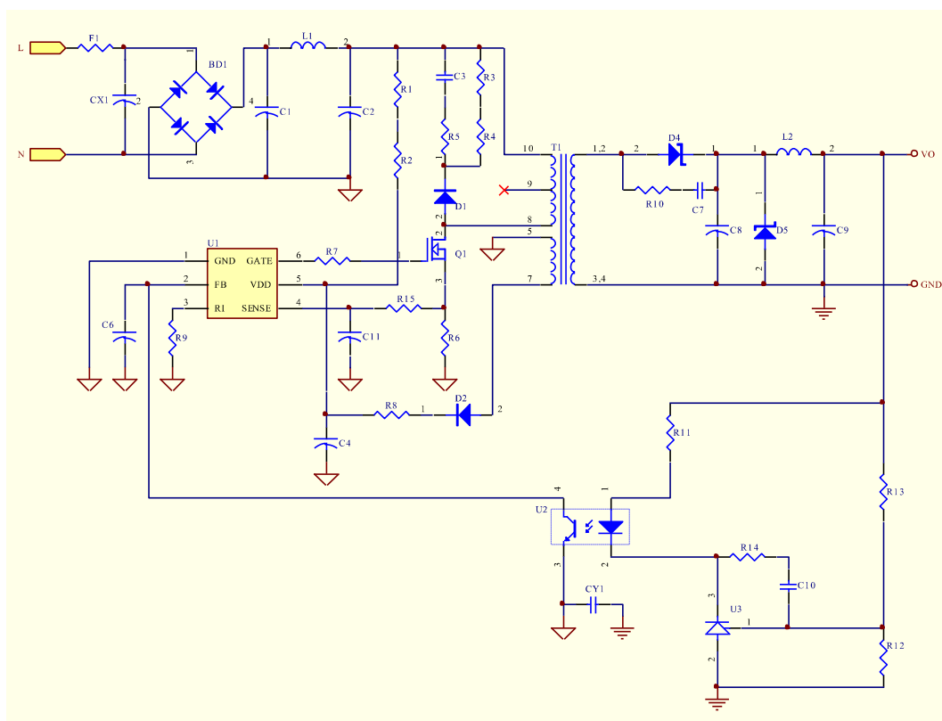
Figure 16. Reference Circuit
