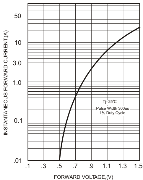
FIG.2-TYPICAL FORWARD CHARACTERISTICS
