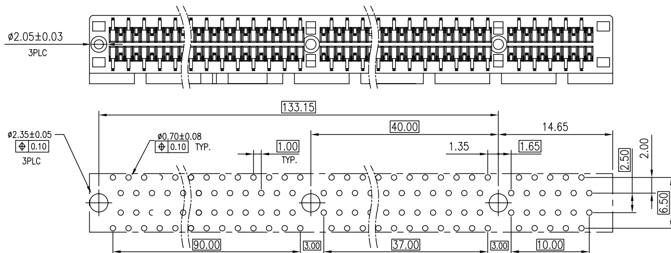
RECOMMENDED PCB LAYOUT(TOP VIEW) PCB TOLERANCE: ±0.05
