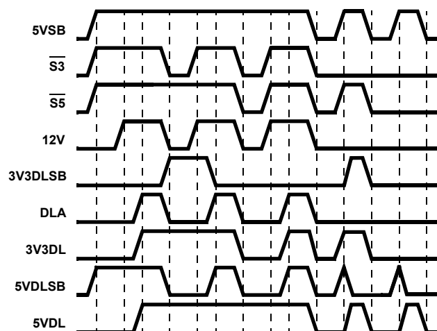
FIGURE 4. 3V_{\text{DUAL}} AND 5V_{\text{DUAL}} TIMING DIAGRAM FOR \text{EN3VDL} = 1 , \text{EN5VDL} = 1
