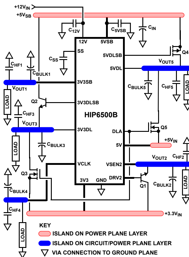
FIGURE 12. PRINTED CIRCUIT BOARD ISLANDS
