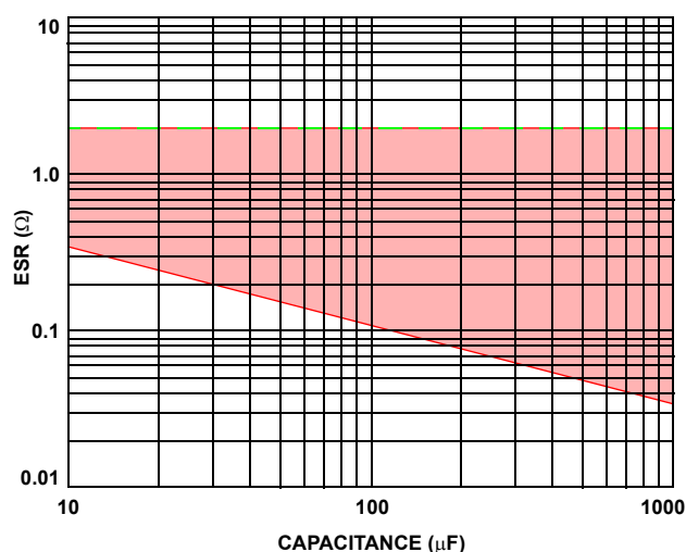
FIGURE 13. C_{OUT4} OUTPUT CAPACITOR
