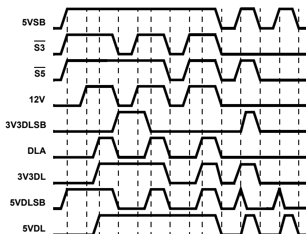
FIGURE 4. 3V_{\text{DUAL}} AND 5V_{\text{DUAL}} TIMING DIAGRAM FOR \text{EN3VDL} = 1 , \text{EN5VDL} = 1
