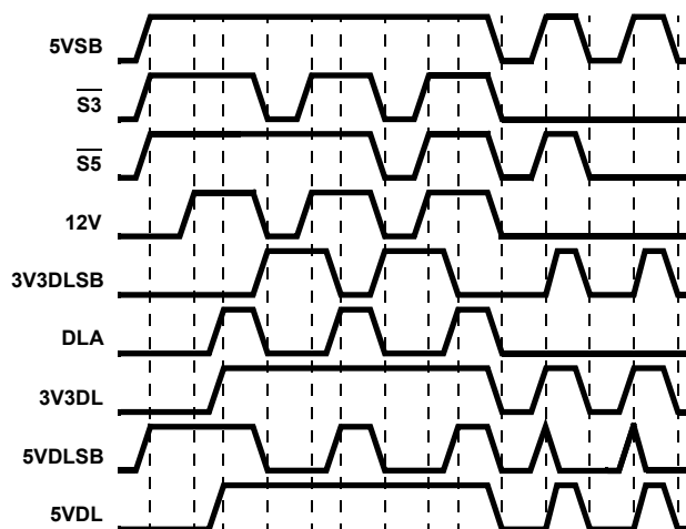
FIGURE 6. 3V_{\text{DUAL}} AND 5V_{\text{DUAL}} TIMING DIAGRAM FOR \text{EN3VDL} = 0 , \text{EN5VDL} = 1
