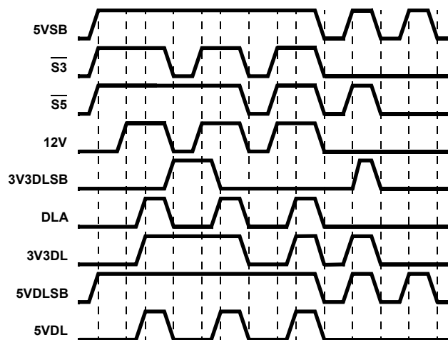
FIGURE 5. 3V_{\text{DUAL}} AND 5V_{\text{DUAL}} TIMING DIAGRAM FOR \text{EN3VDL} = 1 , \text{EN5VDL} = 0
