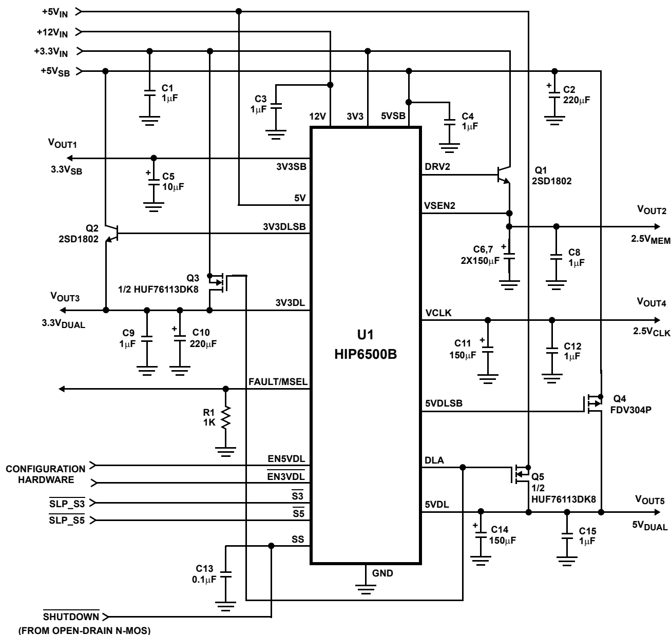
FIGURE 14. TYPICAL HIP6500B APPLICATION DIAGRAM
