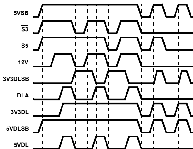
FIGURE 7. 3V_{\text{DUAL}} AND 5V_{\text{DUAL}} TIMING DIAGRAM FOR \text{EN3VDL} = 0 , \text{EN5VDL} = 0
