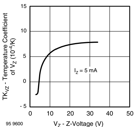
Fig. 3 - Typical Temperature Coefficient of V_Z vs. Z-Voltage
