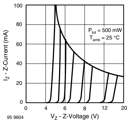
Fig. 5 - Typical Z-Current vs. Z-Voltage
