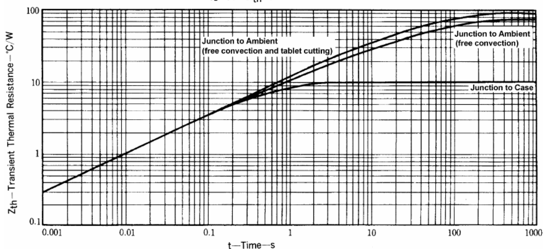
Fig. 11 Z_{th} CHARACTERISTICS
