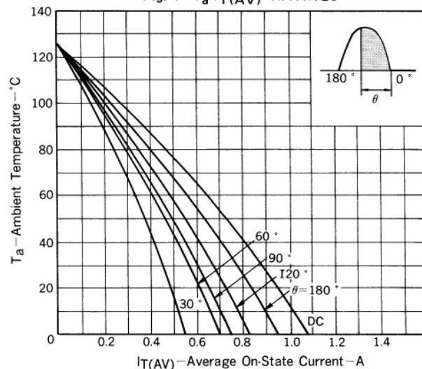
Fig. 4 T_a-I_T(AV) RATINGS
