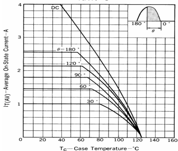
Fig. 3 I_T(AV)-T_C RATINGS
