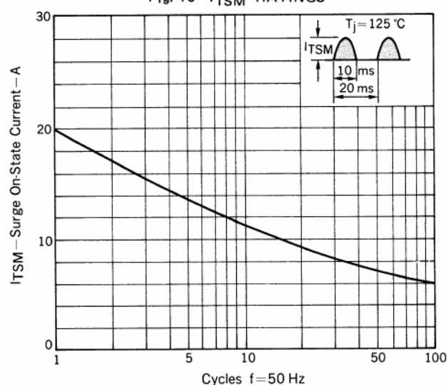
Fig. 10 I_{TSM} RATINGS
