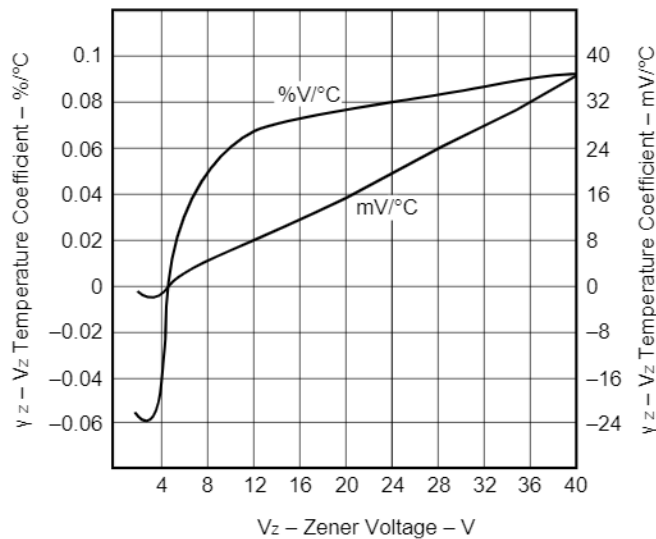
Fig. 3 V_z - V_z CHARACTERISTICS
