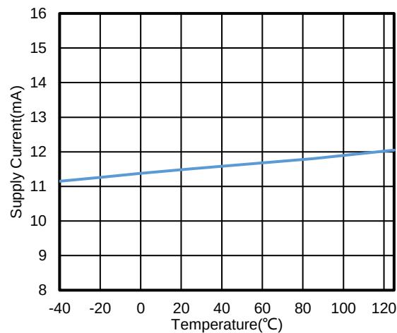
Figure 6. I_q vs. Temperature, \pm 15\text{ V} Supply, TPA2682
