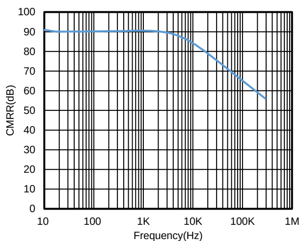
Figure 12. CMRR vs. Frequency
