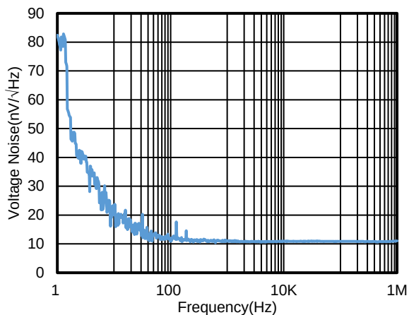
Figure 1. Voltage Noise Density vs. Frequency
