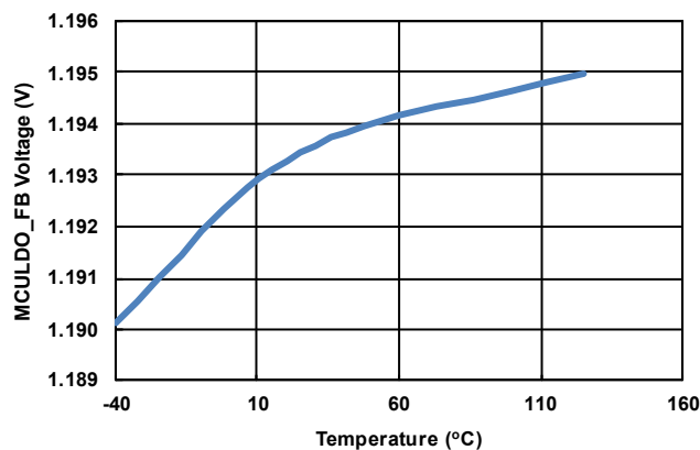
Figure 106. V_{MCU\_LDO\_FB}
