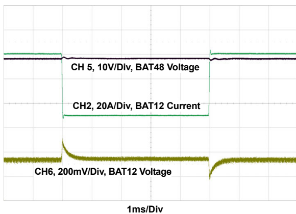
Figure 123. Buck Transient Response 100A to 200A, BAT48 Input ~48V
