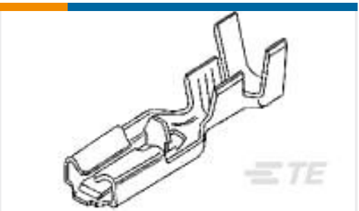
TE Part #63498-1 PL 187 TERMINAL REC 20-16 AWG TPBR
