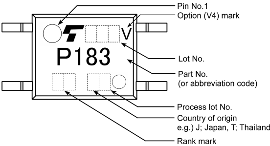
Fig. 15.3 Marking Example (Note)
