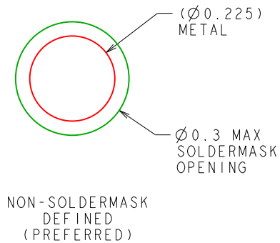
SOLDERMASK DETAILS NOT TO SCALE
