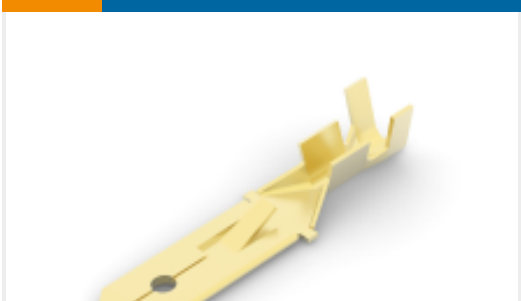
TE Part #880636-1 FF 250 TAB 1.0-2.5 MM2 0.39 X 13.2 BR
