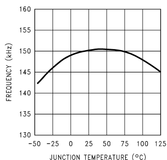
Switching Frequency
