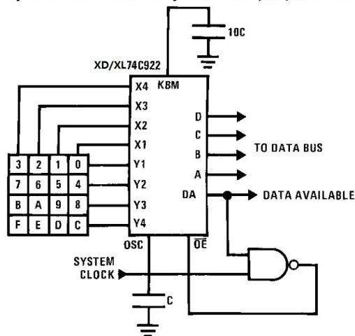
Synchronous Data Entry Onto Bus ( XD/XL74C922)
