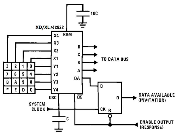
Synchronous Handshake (XD/XL 74C922)
