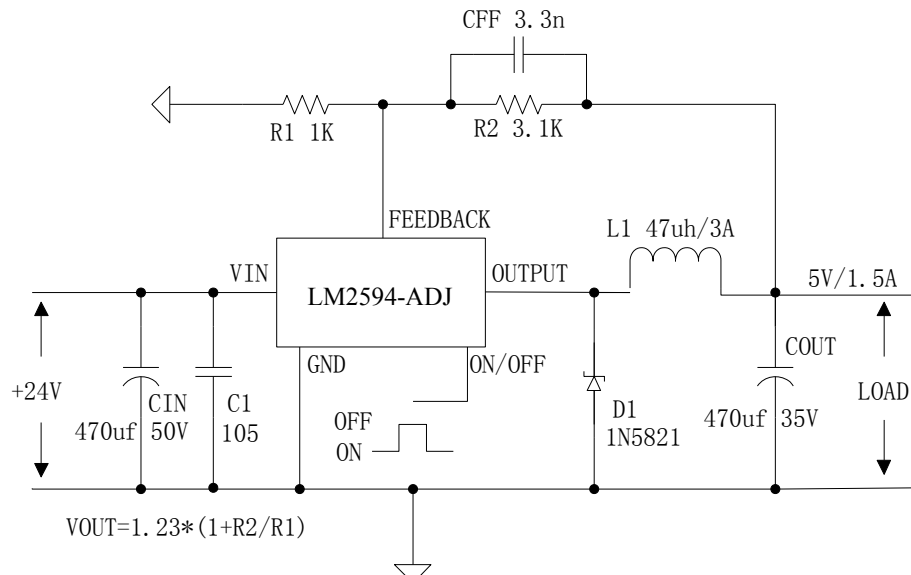
Figure9. LM2594(HV)-ADJ System Parameters Test Circuit
