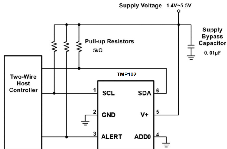
Figure 9. Typical Connections of the UMW TMP102A
