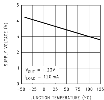
Supply Voltage
