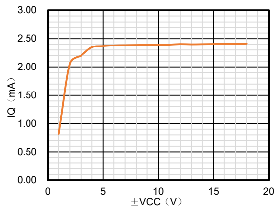
Figure 2. Iq vs. Supply Voltage
