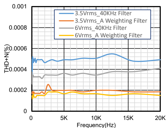
Figure 14. THD vs. Frequency, G = 1
