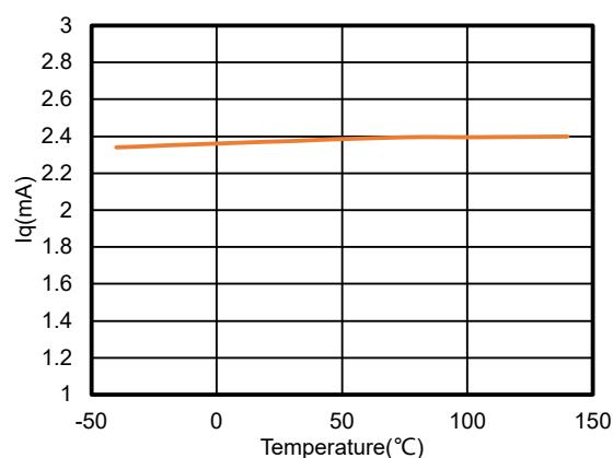
Figure 4. Iq vs. Temperature, +15 V Supply, TPA1862
