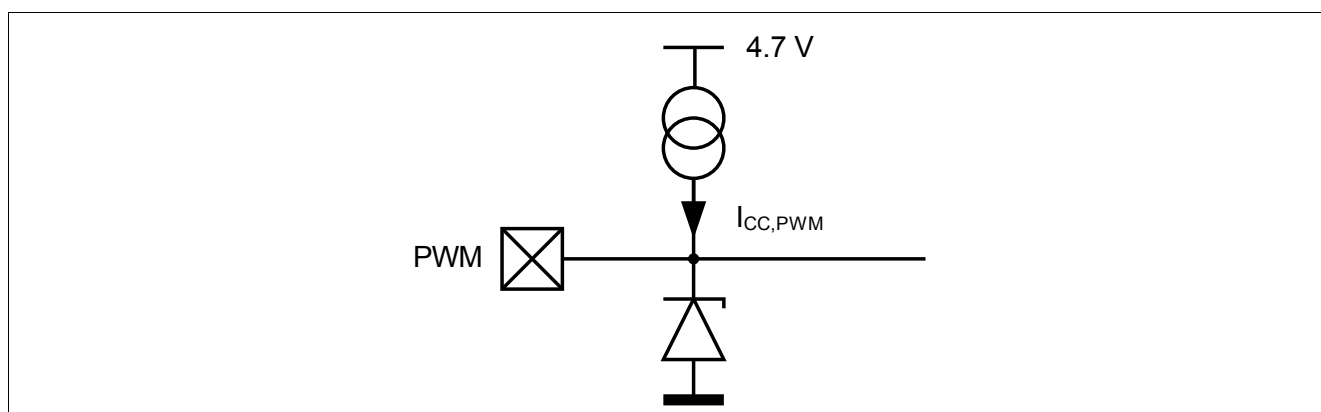
Figure 4 PWM Input
