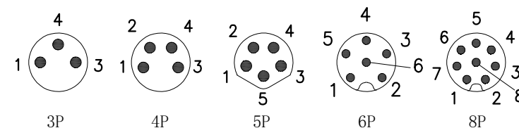
Pin Assignments(Front View)
