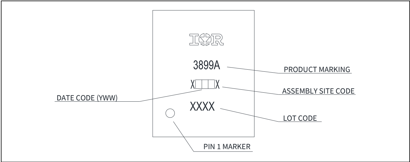
Figure 22 Package Marking
