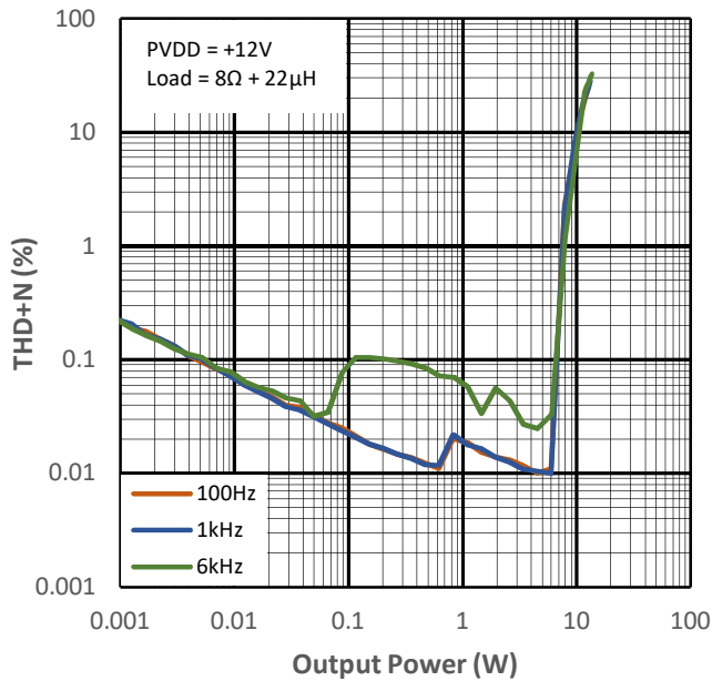
Figure 15-15-1 THD+N vs. Output Power for PMP0
