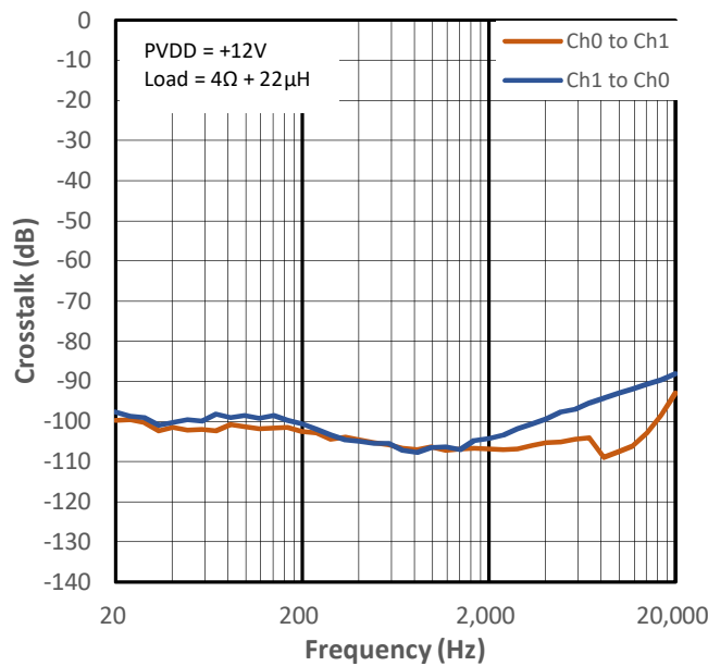
Figure 14-25 Crosstalk vs Frequency for PMP0
