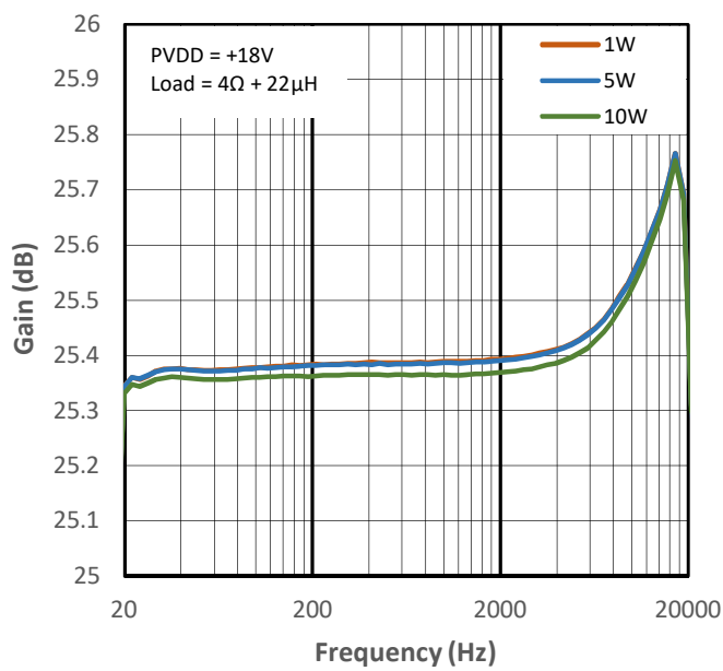
Figure 10-26 Gain vs Frequency for PMP1
