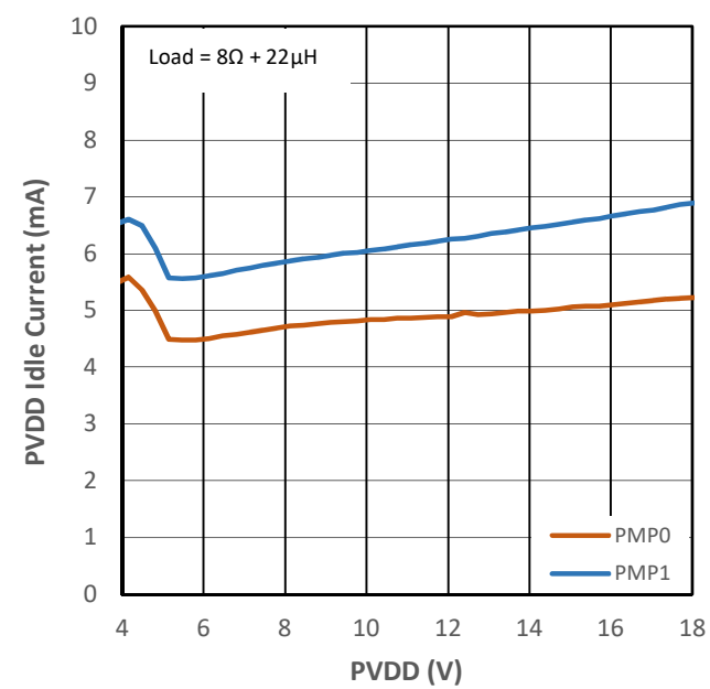
Figure 11-19 PVDD Current vs PVDD Voltage for PMP0 & PMP1
