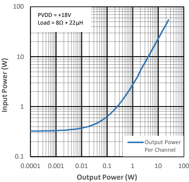
Figure 11-14 Input Power vs Output Power for PMP1
