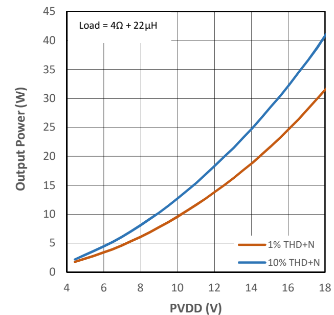
Figure 10-24 Output Power vs PVDD Voltage for PMP4
