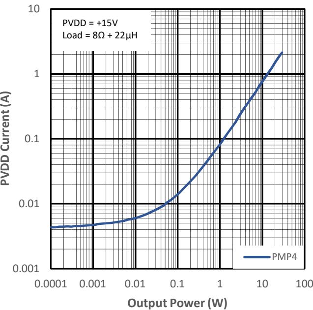
Figure 13-20 PVDD Current vs Output Power for PMP4
