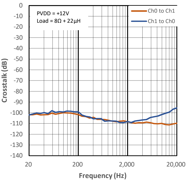
Figure 15-26 Crosstalk vs Frequency for PMP1
