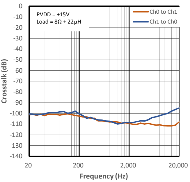
Figure 13-26 Crosstalk vs Frequency for PMP1
