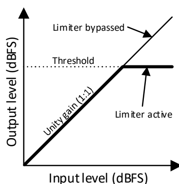
Figure 8-5 Input to Output level characteristic for the Limiter
