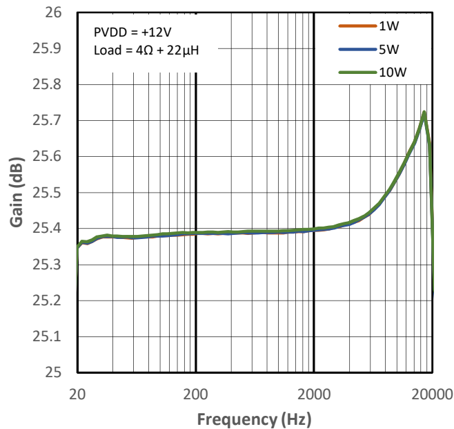
Figure 14-24 Gain vs Frequency for PMP4
