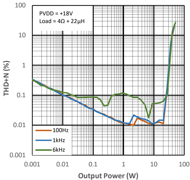
Figure 10-10-1 THD+N vs. Output Power for PMP0
