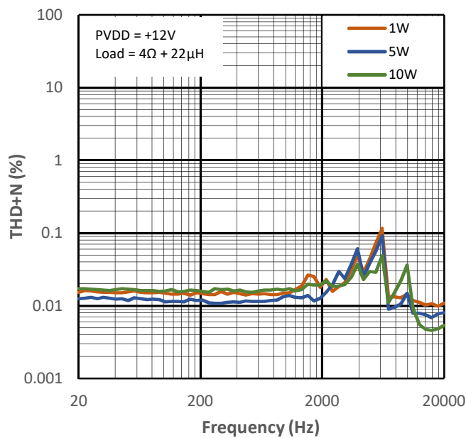
Figure 14-5 THD+N vs Frequency for PMP0
