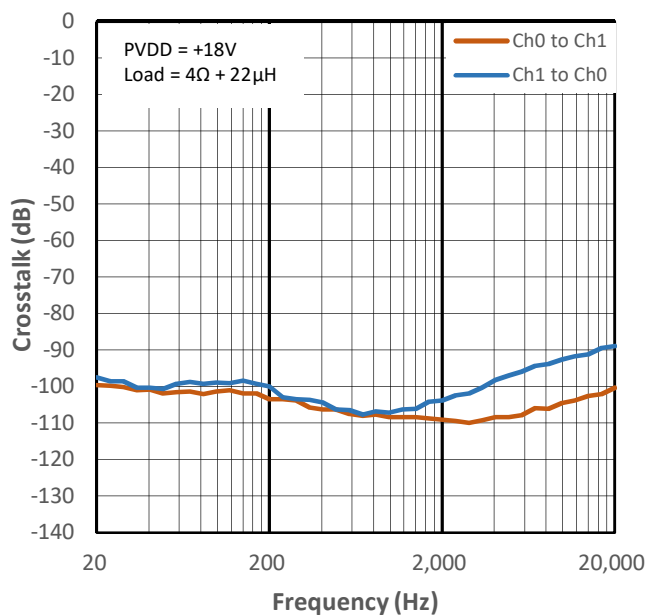
Figure 10-32 Crosstalk vs Frequency for PMP4
