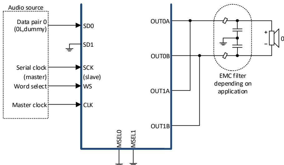
Figure 9-4 Parallel Bridge Tied Load (PBTL) configuration.
