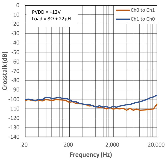
Figure 15-28 Crosstalk vs Frequency for PMP4
