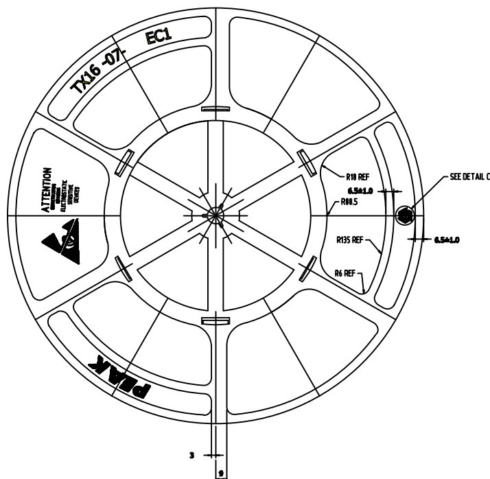
VIEW B
