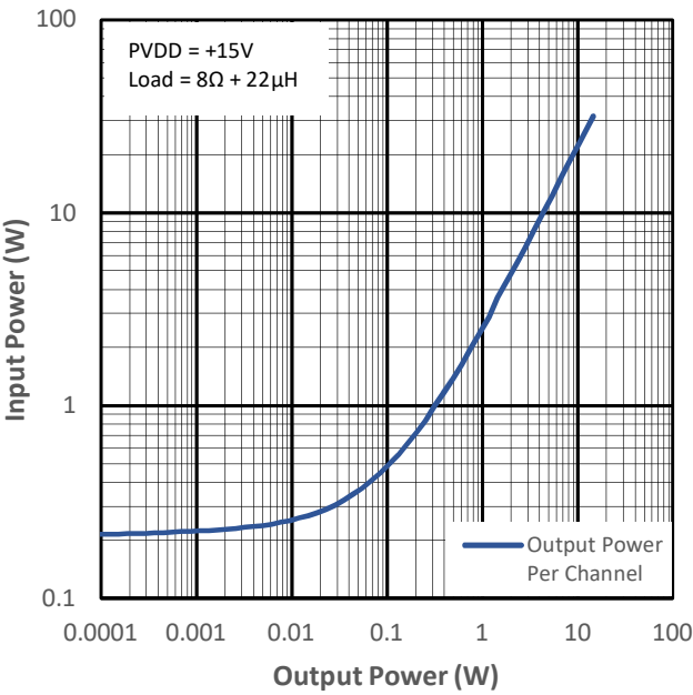
Figure 13-16 Input Power vs Output Power for PMP4
