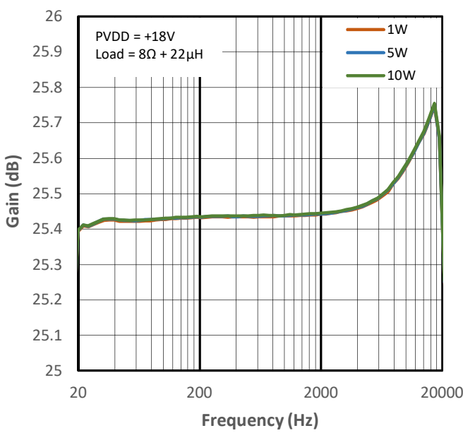
Figure 11-28 Gain vs Frequency for PMP4
