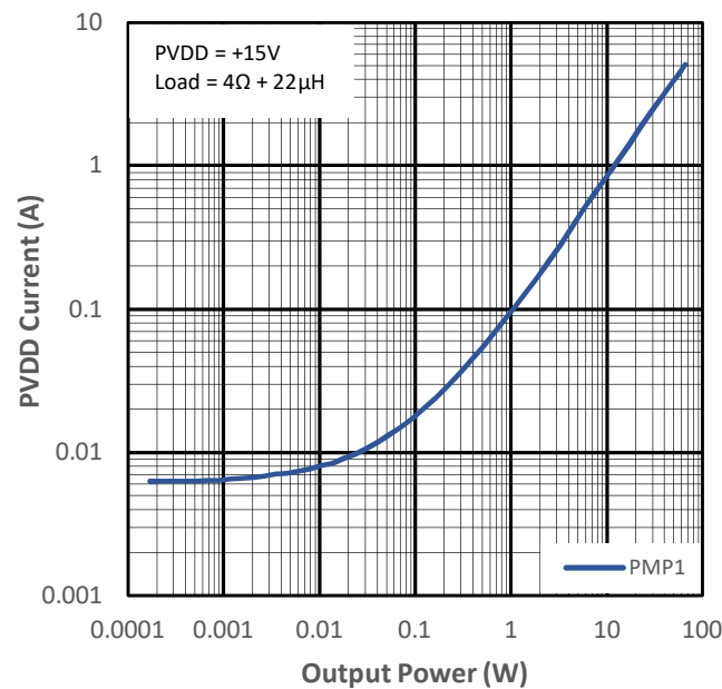
Figure 12-18 PVDD Current vs Output Power for PMP1
