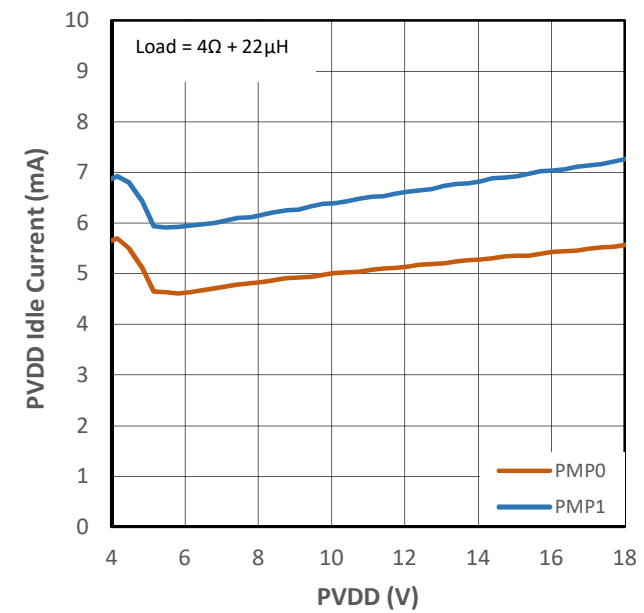
Figure 10-19 PVDD Current vs PVDD Voltage for PMP0 & PMP1
