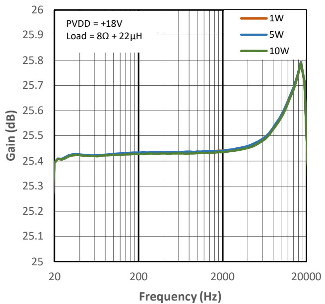
Figure 11-27 Gain vs Frequency for PMP2
