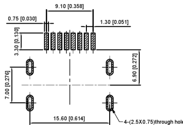
DIMENSIONS OF PC BOARD HOLES TOLERANCE:±0.05(PRINTED-SIDED VIEW)
