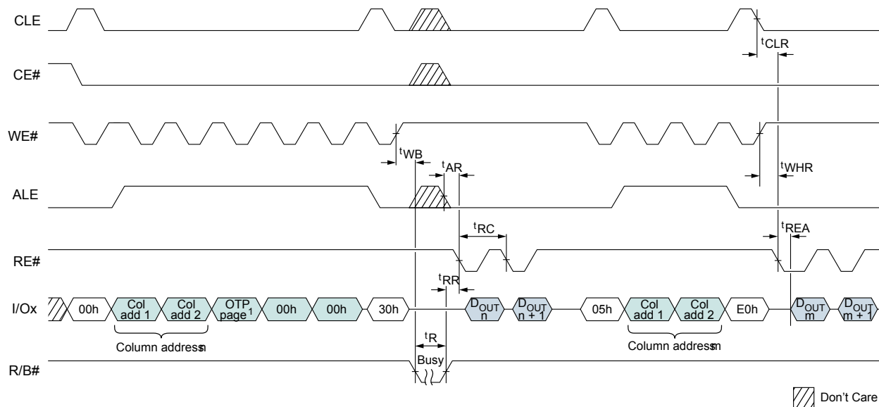
Figure 58: OTP DATA READ with RANDOM DATA READ Operation
