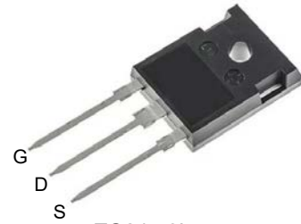
TO247-3L (TO247-3)
